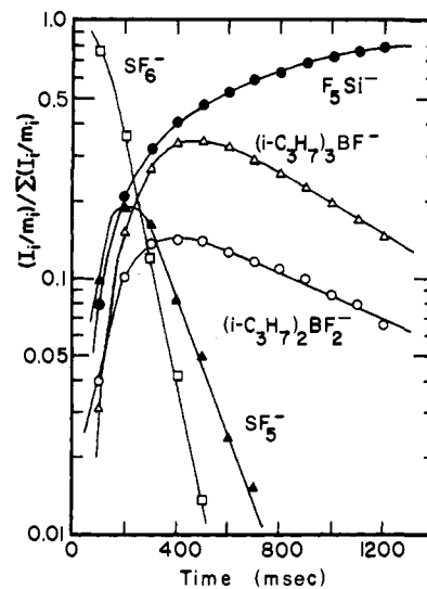
Figure 7. Temporal variation of trapped-anion abundances following a 10-ms 70-eV electron beam pulse in a 3.5:1 mixture of (i\text{-C}_3\text{H}_7)_3\text{B} and \text{SiF}_4 at 9.4 \times 10^{-7} Torr in the presence of trace amounts of \text{SF}_6 .
